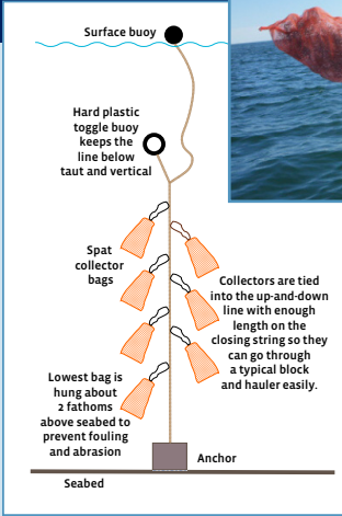
Typical spat line deployment
