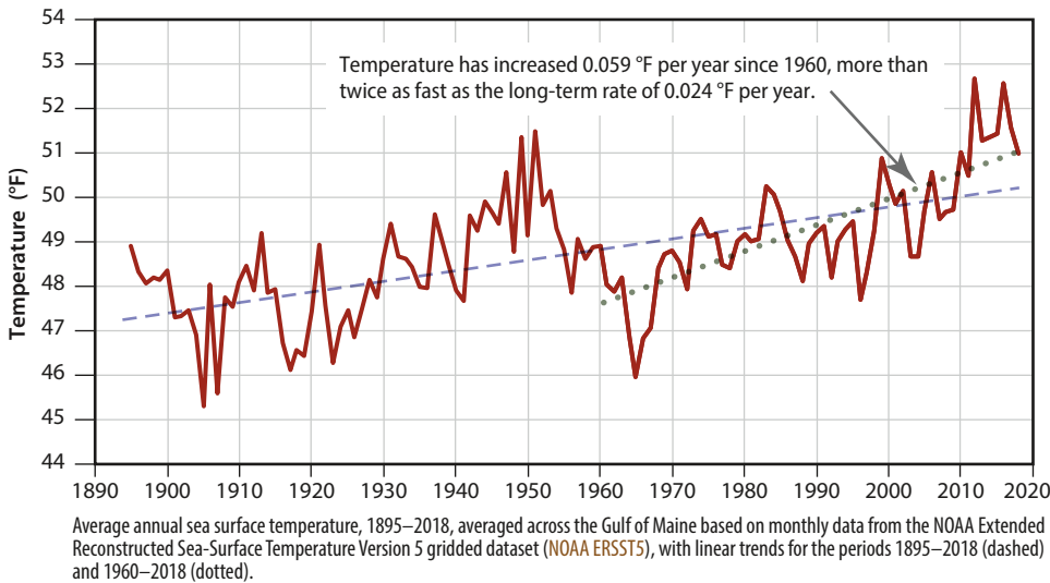
Gulf of Maine Temperature, 1895–2018
