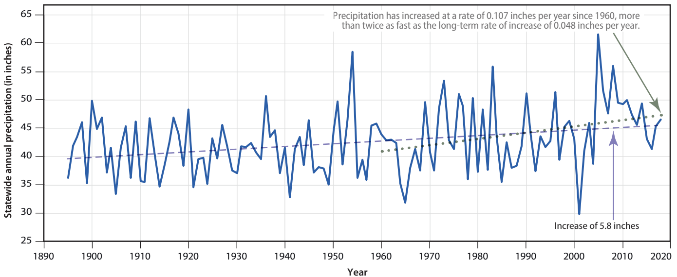
Total annual precipitation, 1895–2018, averaged across Maine based on monthly data from the NOAA U.S. Climate Division Database (NOAA CAAG). Linear trends are depicted for the entire record (dashed) and since 1960 (dotted).
