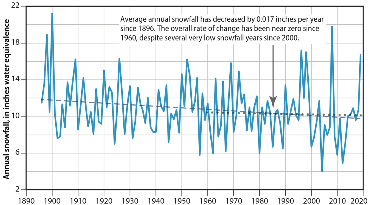
Estimated annual snowfall, 1896-2019, averaged across Maine for the contiguous winter months November-April, with linear trends for the record period (dashed), and since 1960 (dotted). Values derived from monthly temperature and precipitation data from the NOAA U.S. Climate Divisional Database ( NOAA CAAG ), where snow precipitation is assumed for all months (November through April) with a mean temperature of less than 32 °F.
